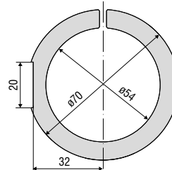
MA 2405-54 for sensors IFS2405-10 IFS2407-3 IFD2415-10
