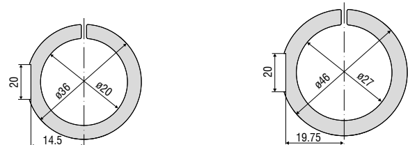
MA 2406-20 for sensors IFS2406-2.5 IFS2406/90-2.5
